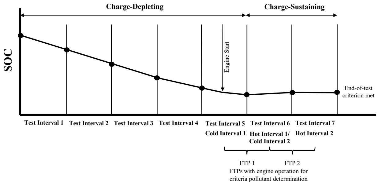
Figure 1 to paragraph (d)(4) of § 1036.512—FTP Charge-Depleting Criteria Pollutant Test Sequence.
